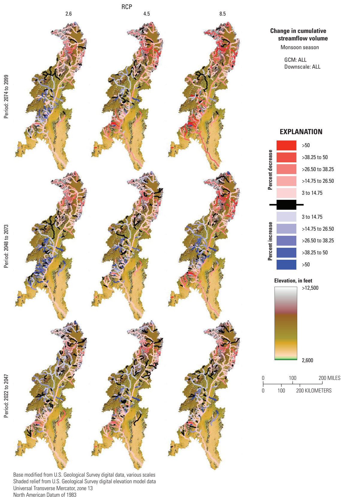
Figure 14. Projected change in cumulative streamflow for all Precipitation-Runoff Modeling System stream segments for monsoon season using the ensemble mean of general circulation models (GCMs) and downscaling scenarios for three future time periods based on the representative concentration pathways (RCPs) 2.6, 4.5, and 8.5 (from van Vuuren and others, 2011; Intergovernmental Panel on Climate Change, 2019).
