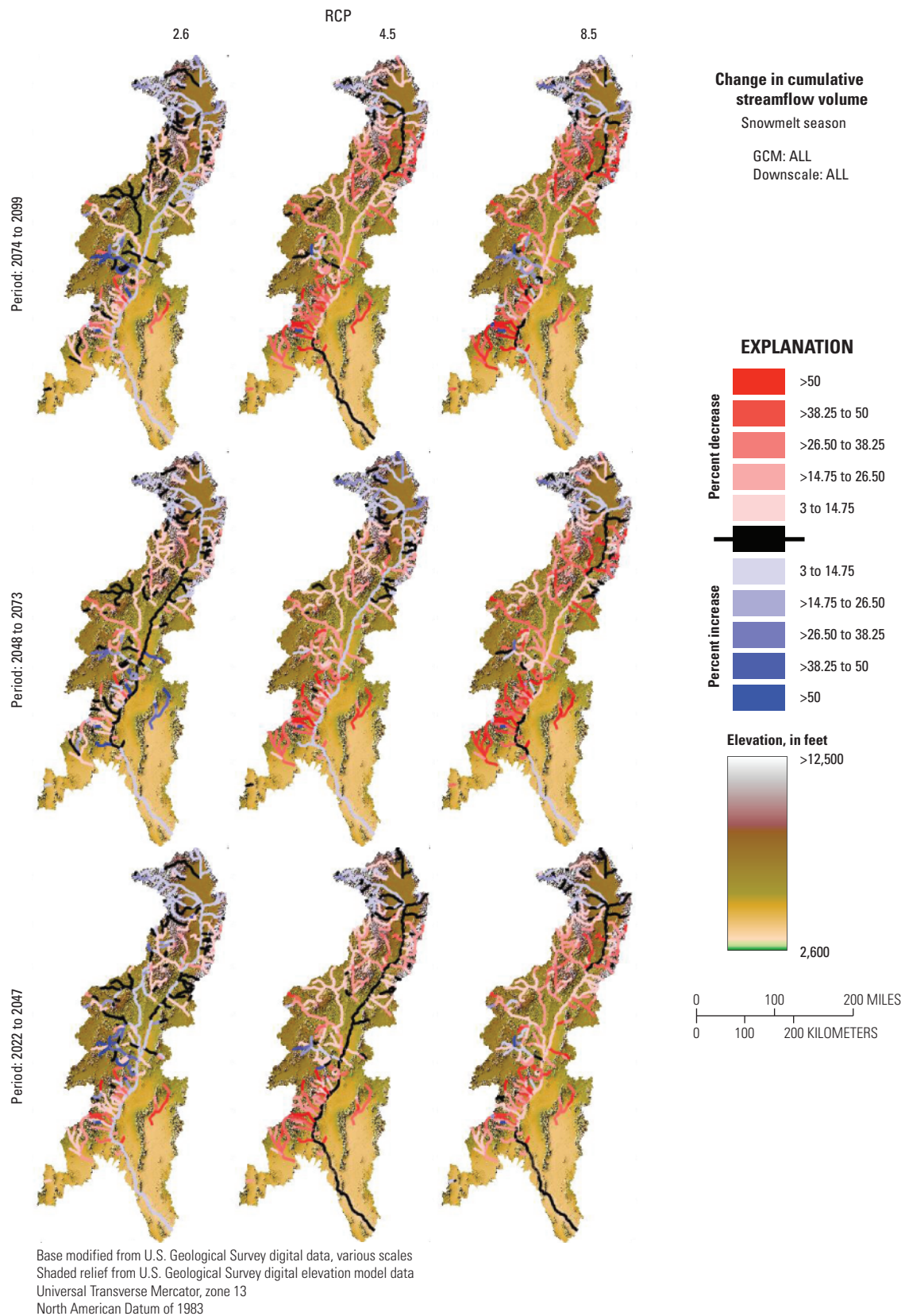
Figure 13. Projected change in cumulative streamflow volume for all Precipitation-Runoff Modeling System stream segments for snowmelt season using the ensemble mean of general circulation models (GCMs) and downscaling scenarios for three future time periods based on the representative concentration pathways (RCPs) 2.6, 4.5, and 8.5 (from van Vuuren and others, 2011; Intergovernmental Panel on Climate Change, 2019).
