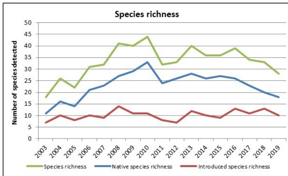
Figure 23. Plant species richness from 2003 to 2019.
