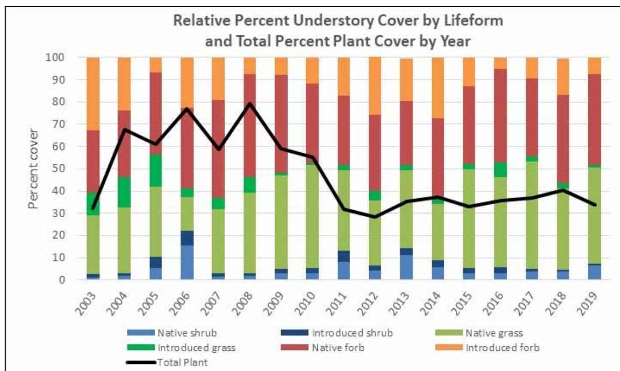
Figure 24. Relative percent cover by life-form and total plant cover (black line) in the understory layer from 2003 to 2019.
