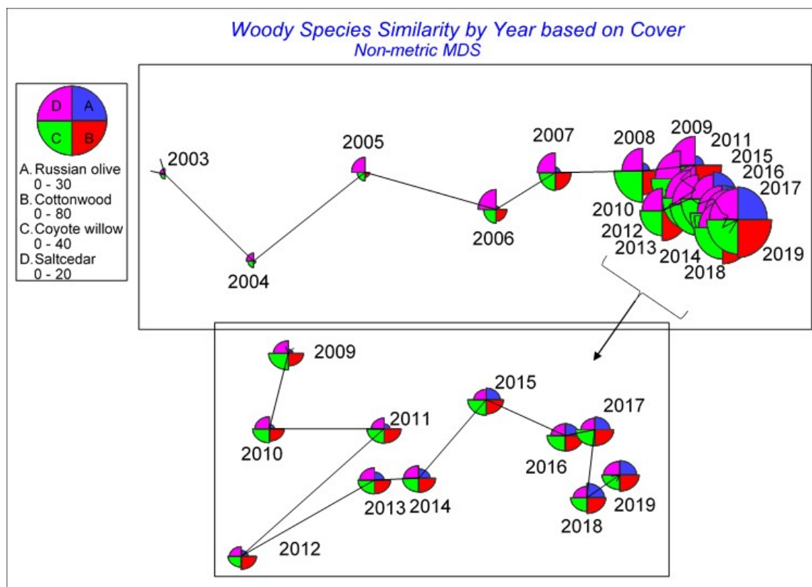
Figure 28. MDS ordination of 17 years of woody plant species cover data based on Bray-Curtis similarities (stress=0.01). Overlay circles associated with each year represent percent cover of 4 dominant overstory species.
