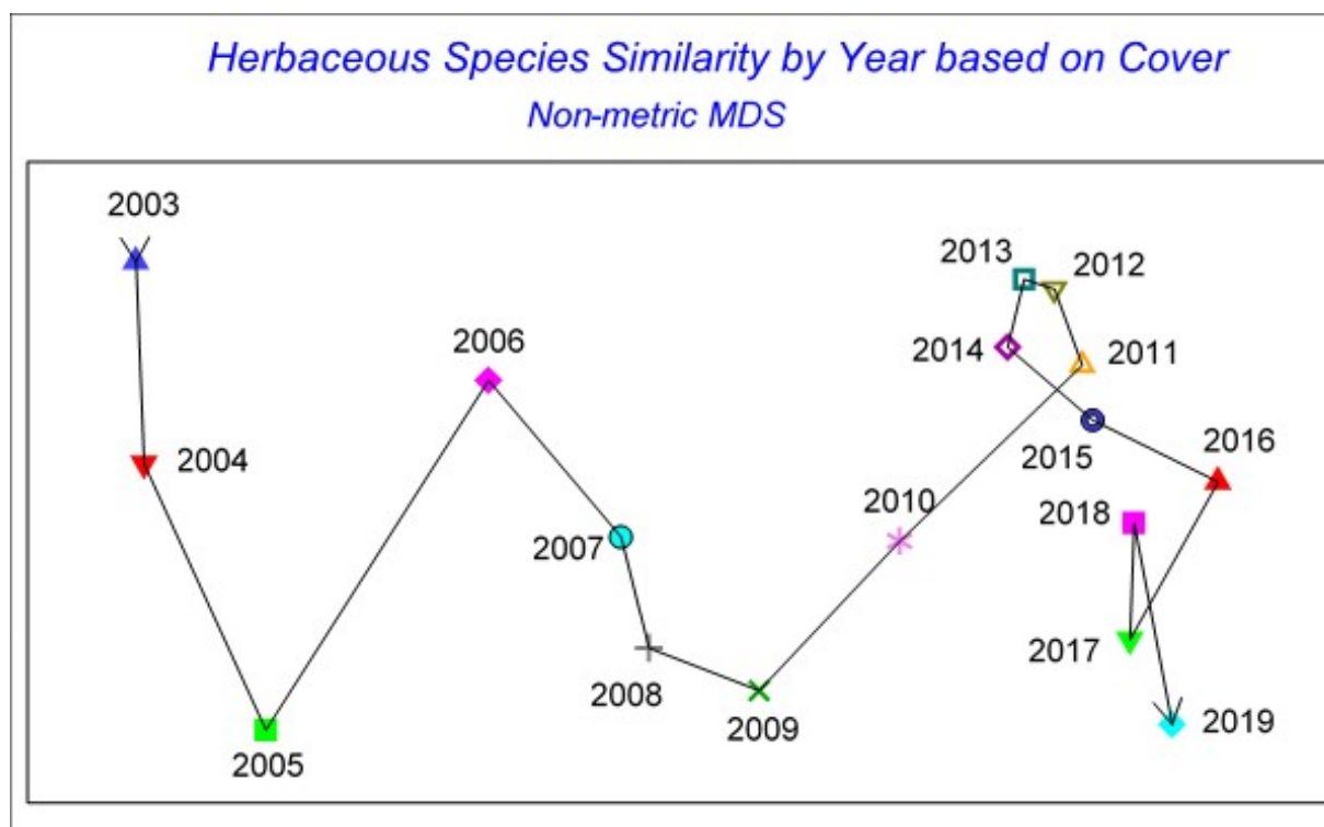
Figure 27. MDS ordination of 17 years of understory plant species 4 th root transformed cover data based on Bray-Curtis similarities (stress=0.06).
