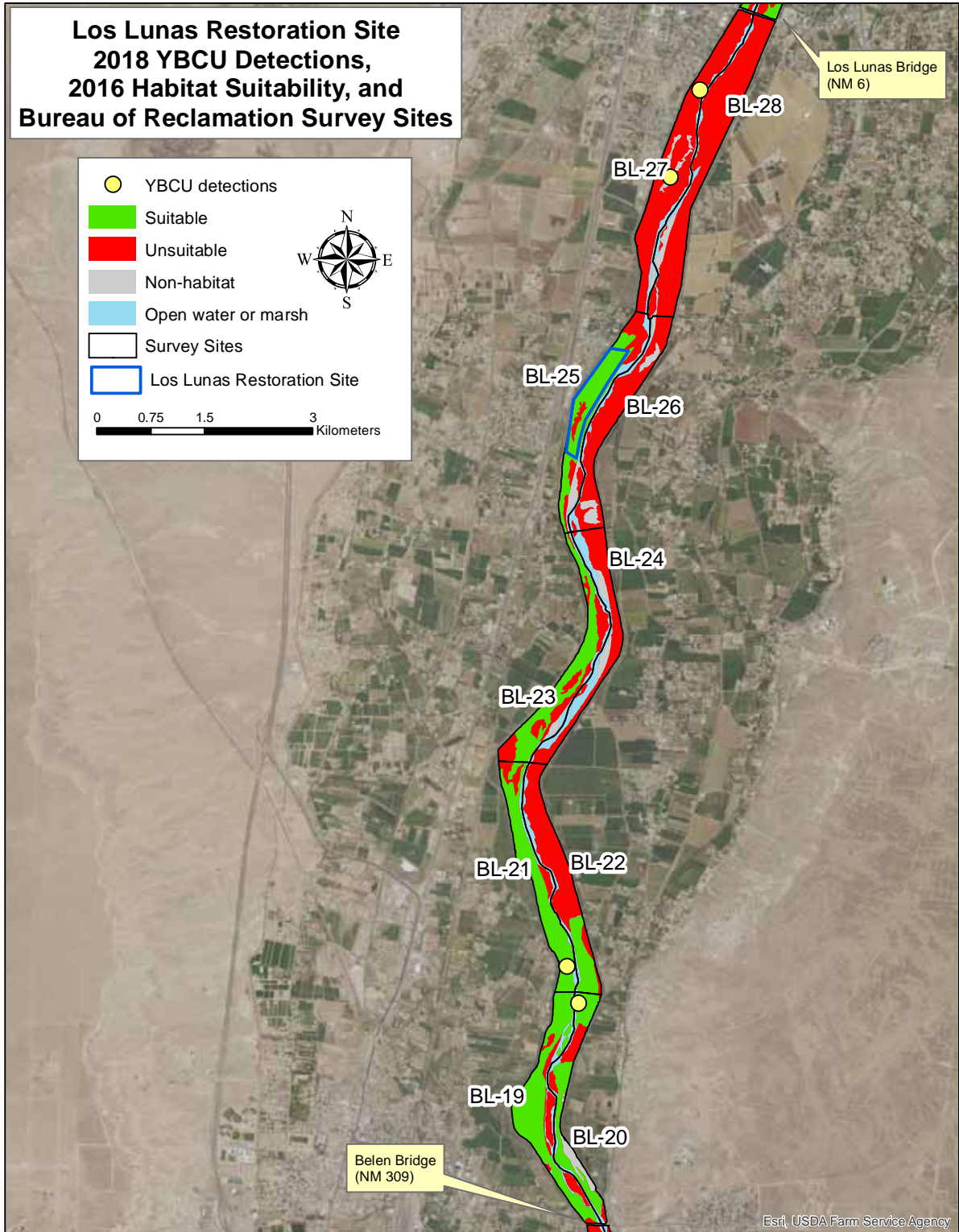
Figure 20. 2018 YBCU detections and habitat suitability in the vicinity of LLRS within the Belen survey site.
