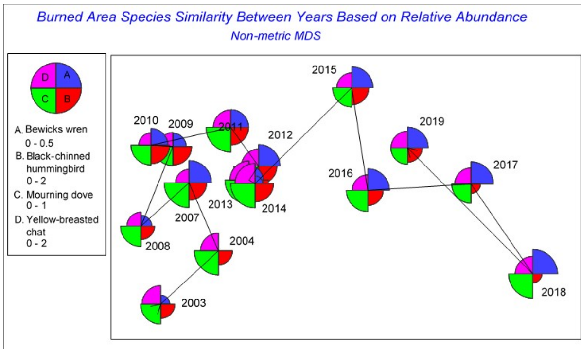
Figure 13. MDS ordination of 15 years of square root transformed species abundance data based on Bray Curtis similarities within the Burned Area (stress=0.09). Overlay circles associated with each year represent relative abundance of 4 of the species detected.
