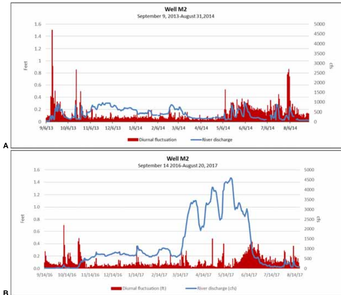
Figure 30. Examples of diurnal fluctuation (ft) within Well M2 and average discharge (cfs) in the Rio Grande at Bosque Farms, New Mexico from September through August (A) 2013-2014 and (B) 2016 – 2017.
