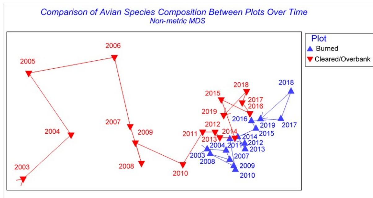
Figure 16. MDS ordination based on 17 years of square root transformed species abundance data and Bray-Curtis similarities for both the Cleared/Overbank and Burned Areas; 2D stress=0.08.
