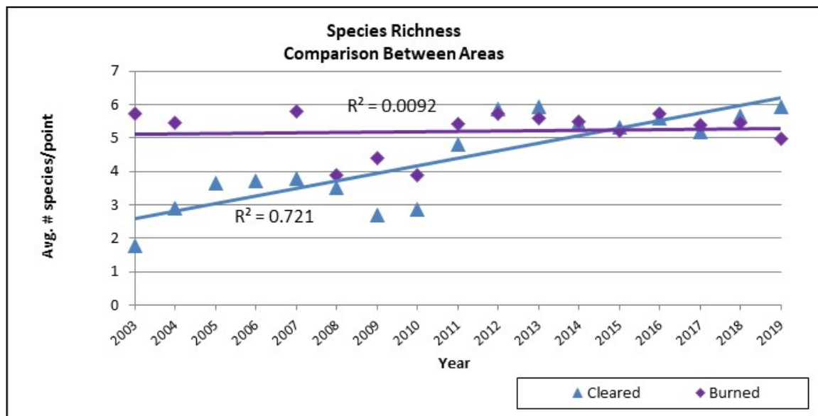
Figure 18. Trendlines and R 2 values for species richness over time in the Cleared/Overbank Area (2003-2019) and Burned Area (2003, 2004, 2007-2019).
