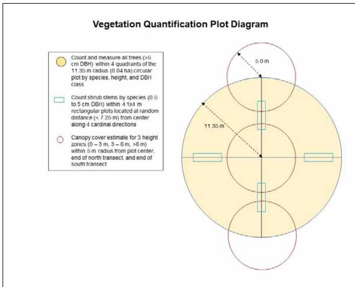
Figure 6. Vegetation quantification plot layout.
