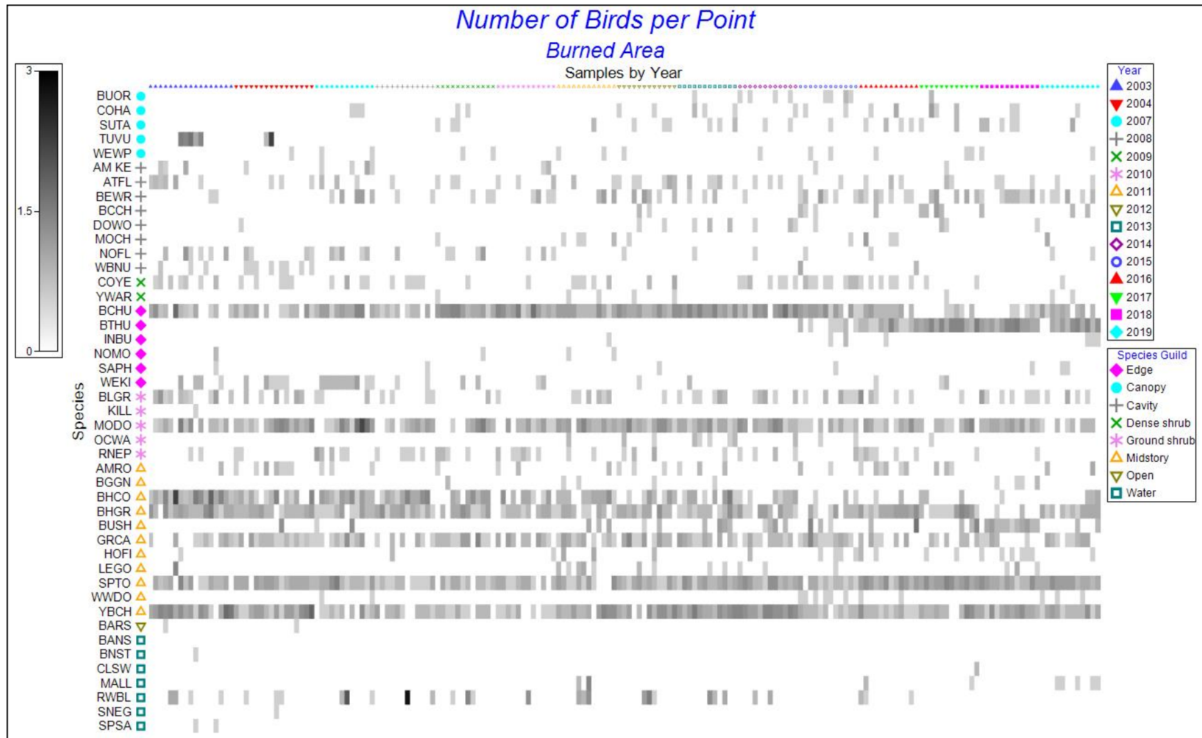
Figure 12. Shade plot of the most abundant species detected in the Burned Area by sample and year; darker shades in each cell represent higher abundance of that species. See Appendix B for species code.
