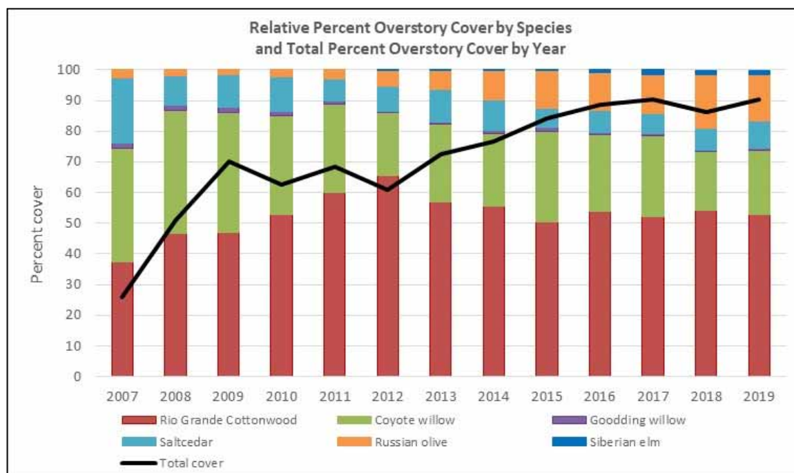
Figure 25. Total percent cover of overstory species (woody species > 1 m) by species from 2007 to 2019.
