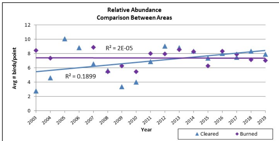
Figure 17. Trendlines and R 2 values for relative abundance over time in the Cleared/Overbank Area (2003-2019) and Burned Area (2003, 2004, 2007-2019).
