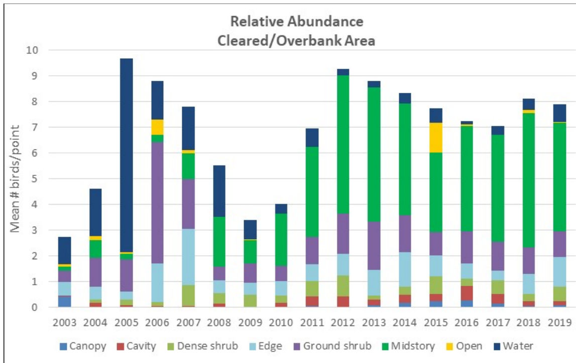
Figure 9. Relative abundance by species guilds in the Cleared/Overbank Area over time.
