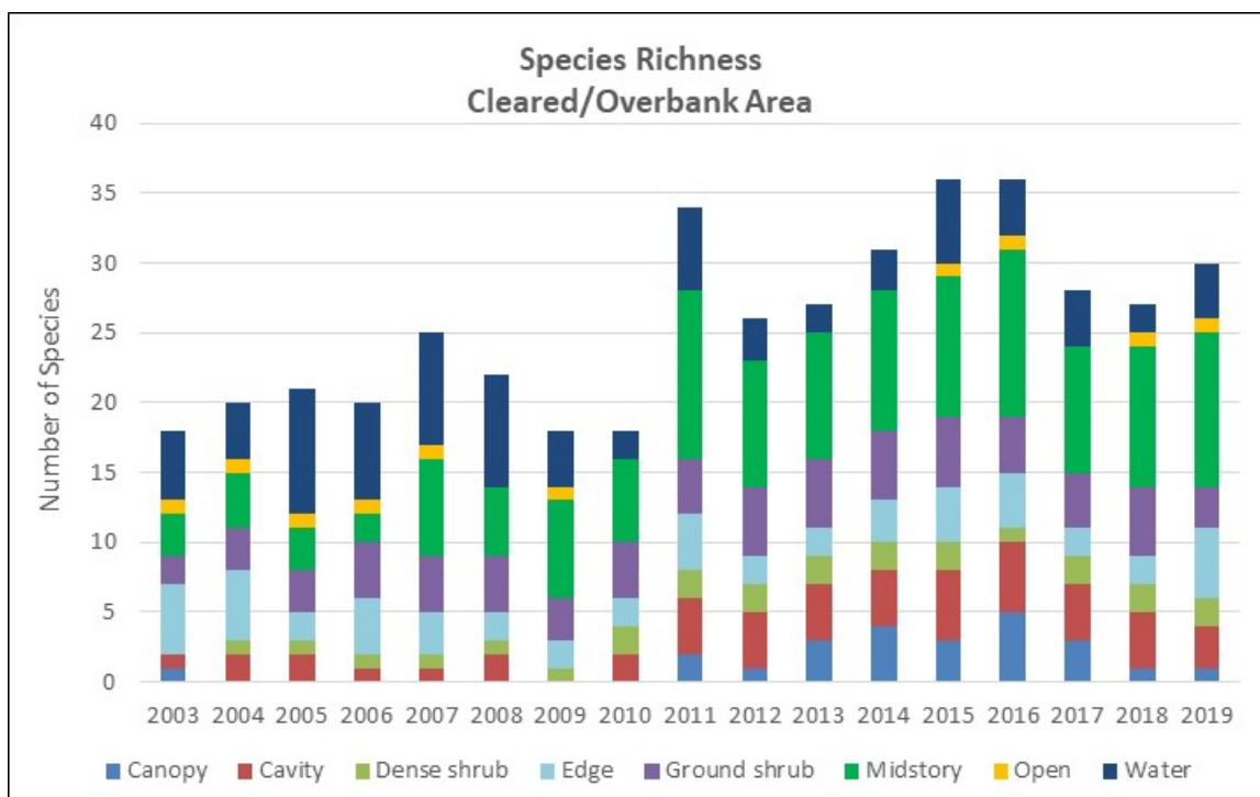
Figure 10. Species richness by species guilds in the Cleared/Overbank Area over time.
