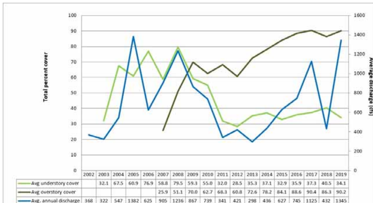
Figure 29. Hydrologic year (Oct–Sept) average discharge (cfs) in the Rio Grande at San Acacia (2002-2007) and at Bosque Farms (2008-2019), and the average total percent plant cover in transects at the LLRS. Restoration occurred in 2002; vegetation monitoring began in 2003. Overstory was not a separate cover measurement until 2007.
