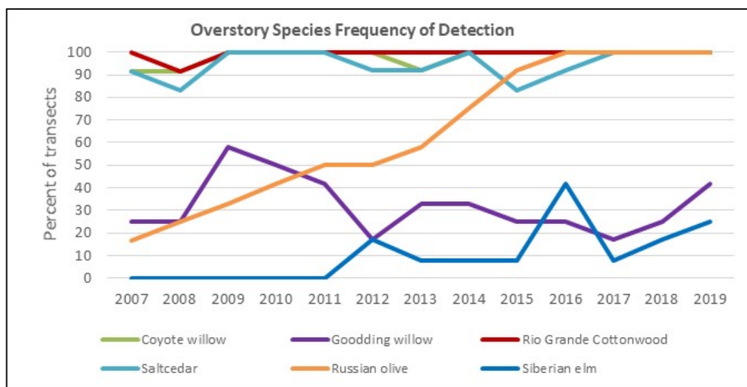
Figure 26. Percentage of transects in which overstory species were detected from 2007 to 2019.
