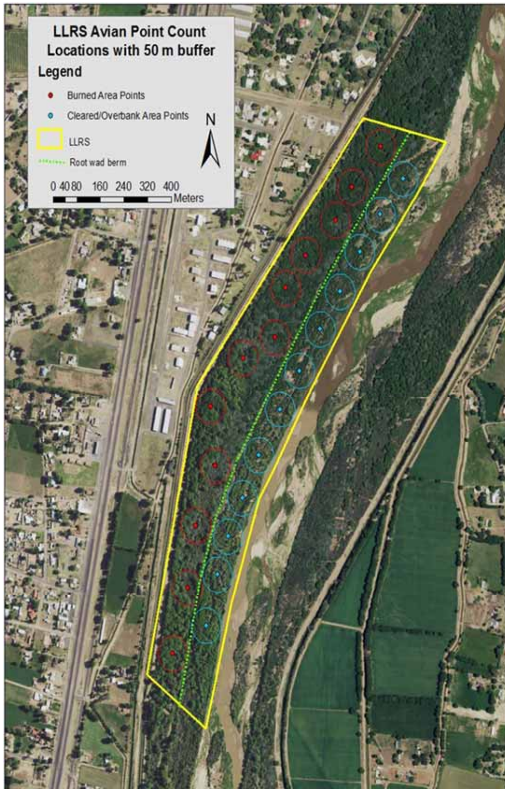
Figure 2. Cleared/Overbank and Burned Area point count locations at LLRS. A root wad berm separates the 2 areas.
