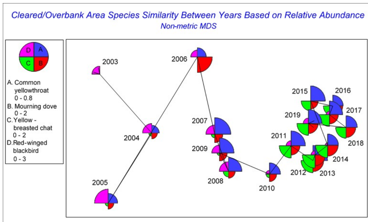
Figure 8. MDS ordination of 17 years of square root transformed species abundance data based on Bray-Curtis similarities within the Cleared/Overbank Area (stress=0.07). Overlay circles associated with each year represent relative abundance of 4 of the species detected.
