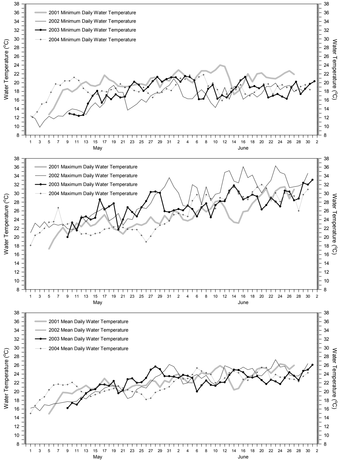
Figure 10. Comparisons of annual minimum, maximum, and mean daily water temperatures during the 2001-04 Rio Grande silvery minnow spawning periodicity study periods.
