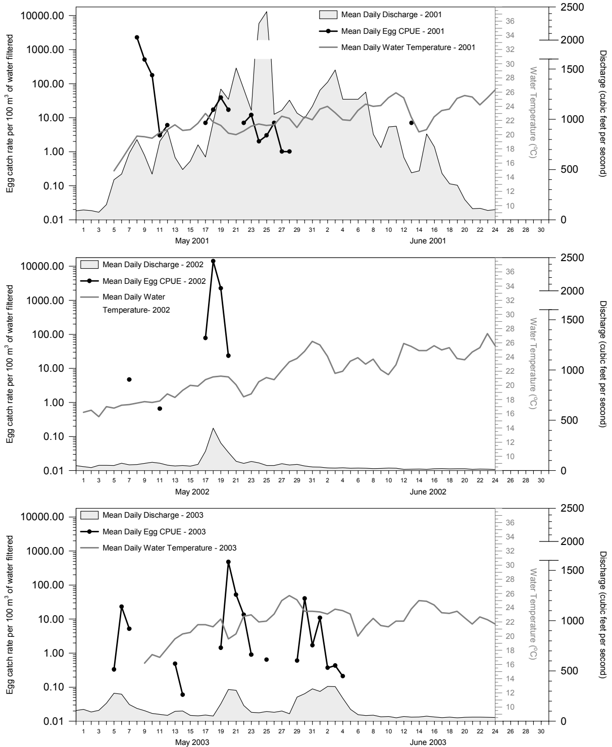
Figure 8. Mean daily discharge (San Marcial), mean daily egg catch rate, and mean daily water temperature during the 2001-03 Rio Grande silvery minnow spawning periodicity study periods. Note that the Y-axis for egg catch rate is a log-scale.
