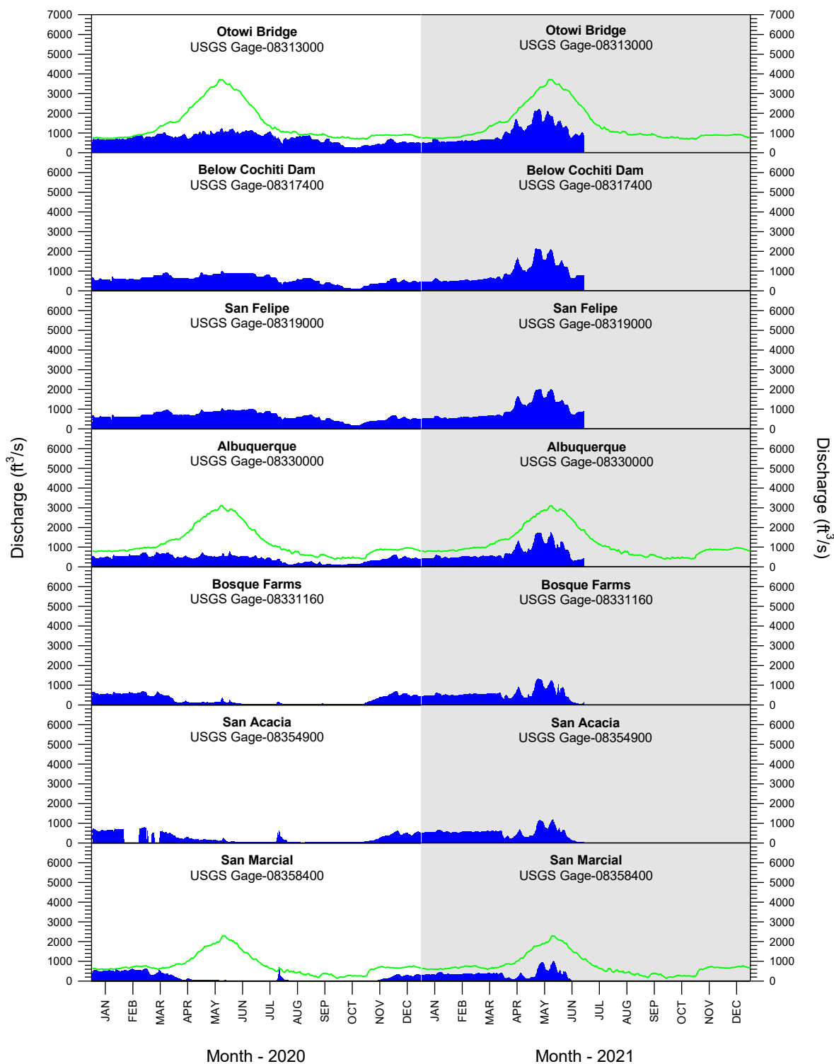
Figure 2. Rio Grande mean-daily discharge, by USGS gaging station, from 1 January 2020 to 30 June 2021. Green lines are the average mean-daily discharges across years (1973–2020).
