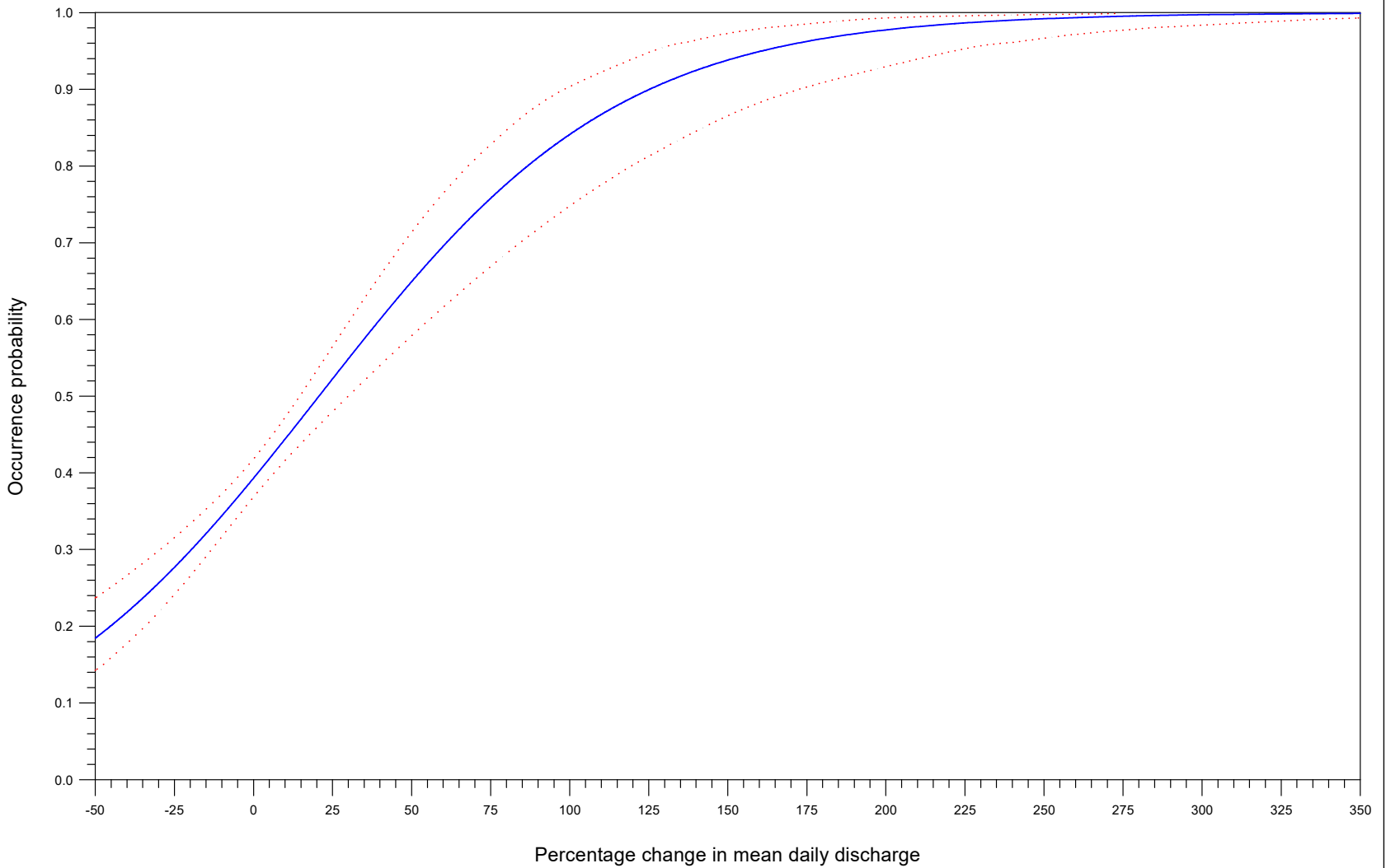
Figure 6. Logistic regression plot, using data from all sites (22 April to 10 June; 2003–2021), illustrating Rio Grande Silvery Minnow daily egg-occurrence probability as a function of the percentage change in mean daily discharge taken from the nearest upstream gaging station. Logistic regression line (solid) and 95% confidence intervals (dotted) are illustrated.
