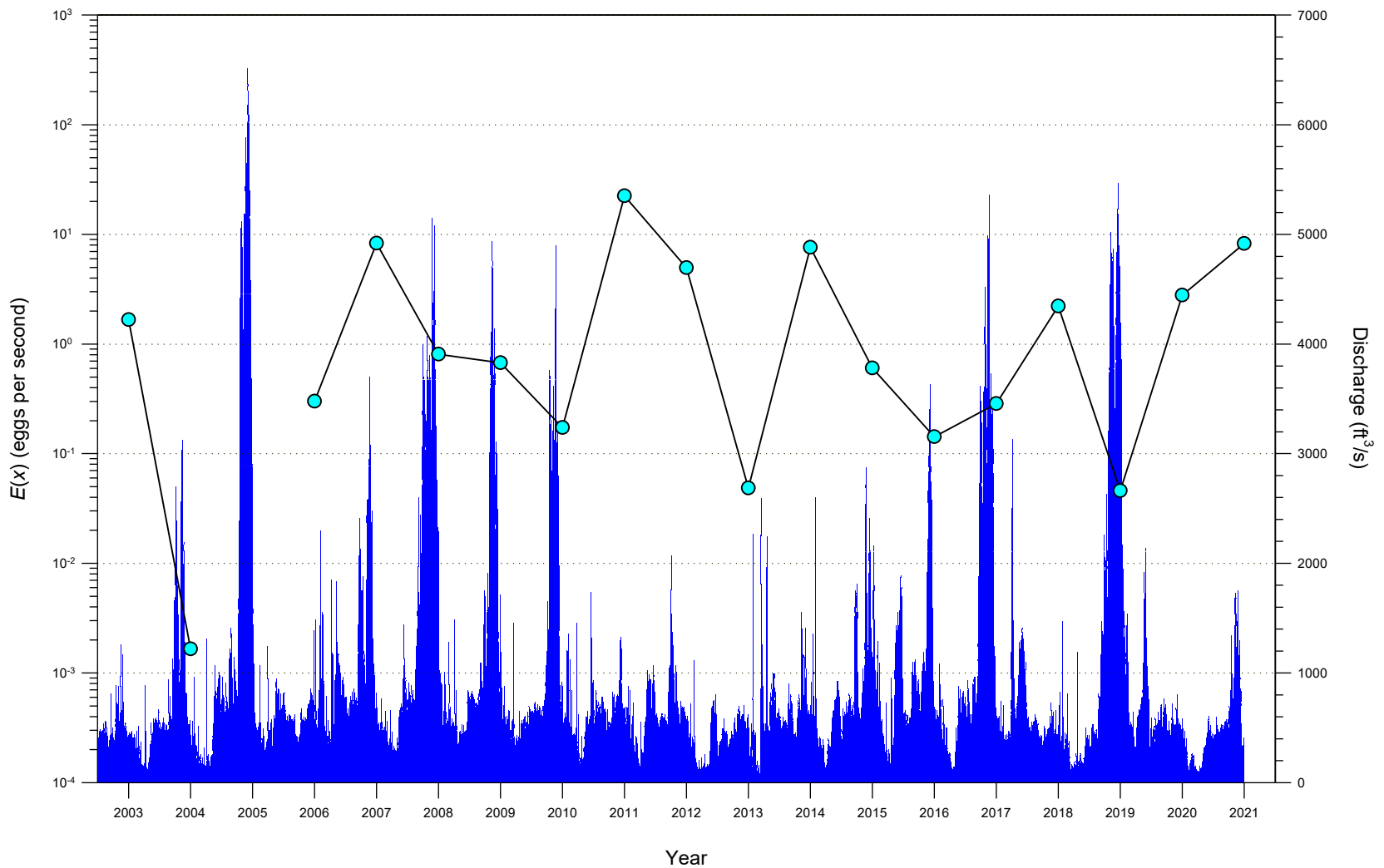
Figure 8. Rio Grande Silvery Minnow egg-passage rates (estimated using data from all sites [22 April to 10 June]), and mean daily discharge data from the Albuquerque Gage (2003-01-01 to 2021-06-30), across years. Sampling did not occur in 2005.
