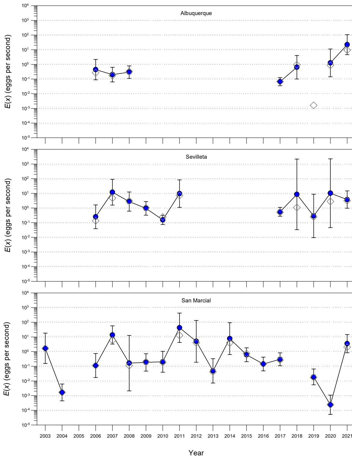
Figure 4. Rio Grande Silvery Minnow egg-passage rates (estimated using 22 April to 10 June data) across sites and years. Modeled estimates (circles), 95% confidence intervals (bars), and method-of-moments estimates (diamonds) are illustrated.
