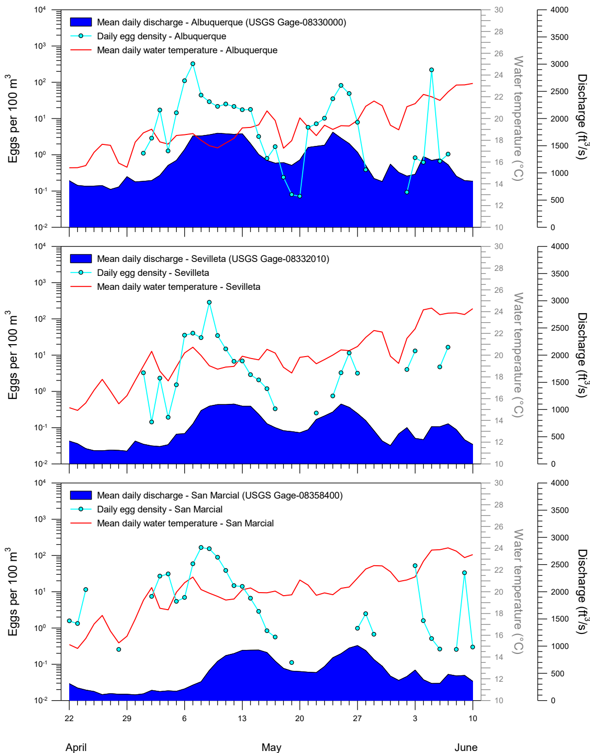
Figure 3. Mean daily discharge, daily egg density, and mean daily water temperature, by site and date, during 2021 (see Table 1 for egg abundance data).
