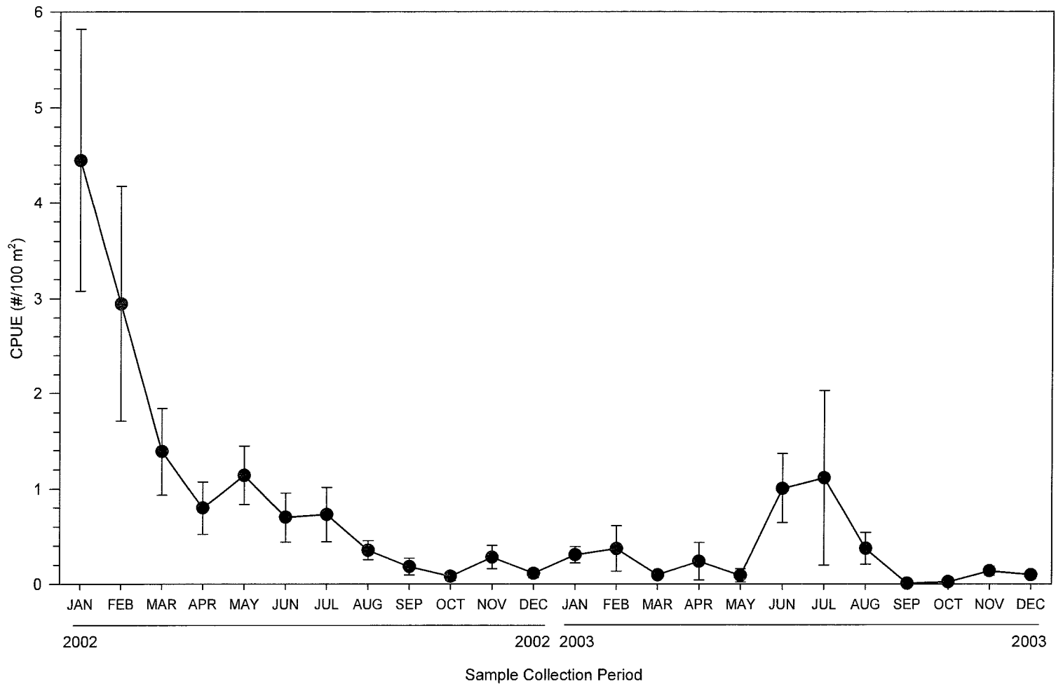
Figure 11. Monthly catch rates of Rio Grande silvery minnow during 2002 (January-December) and through December 2003 at population monitoring program collection sites. Solid circles indicate monthly means (n=20 sites per month) and capped-bars represent the standard error.
