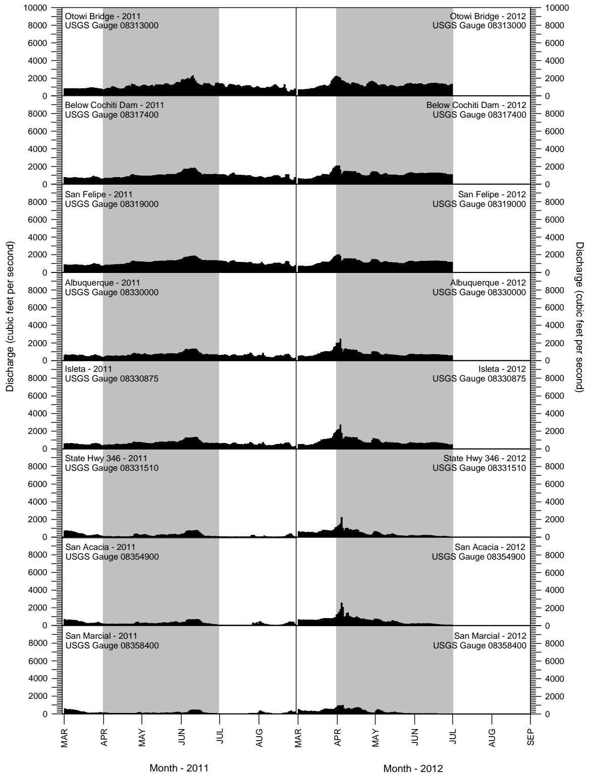
Figure 7. Rio Grande discharge from March through August 2011 and March through June 2012 at seven U. S. Geological Survey Gauging Stations (see Figure 1). The Otowi Bridge gauge is not shown in Figure 1 but is provided for reference. Gray rectangles indicate peak months for Rio Grande silvery minnow spawning activity.
