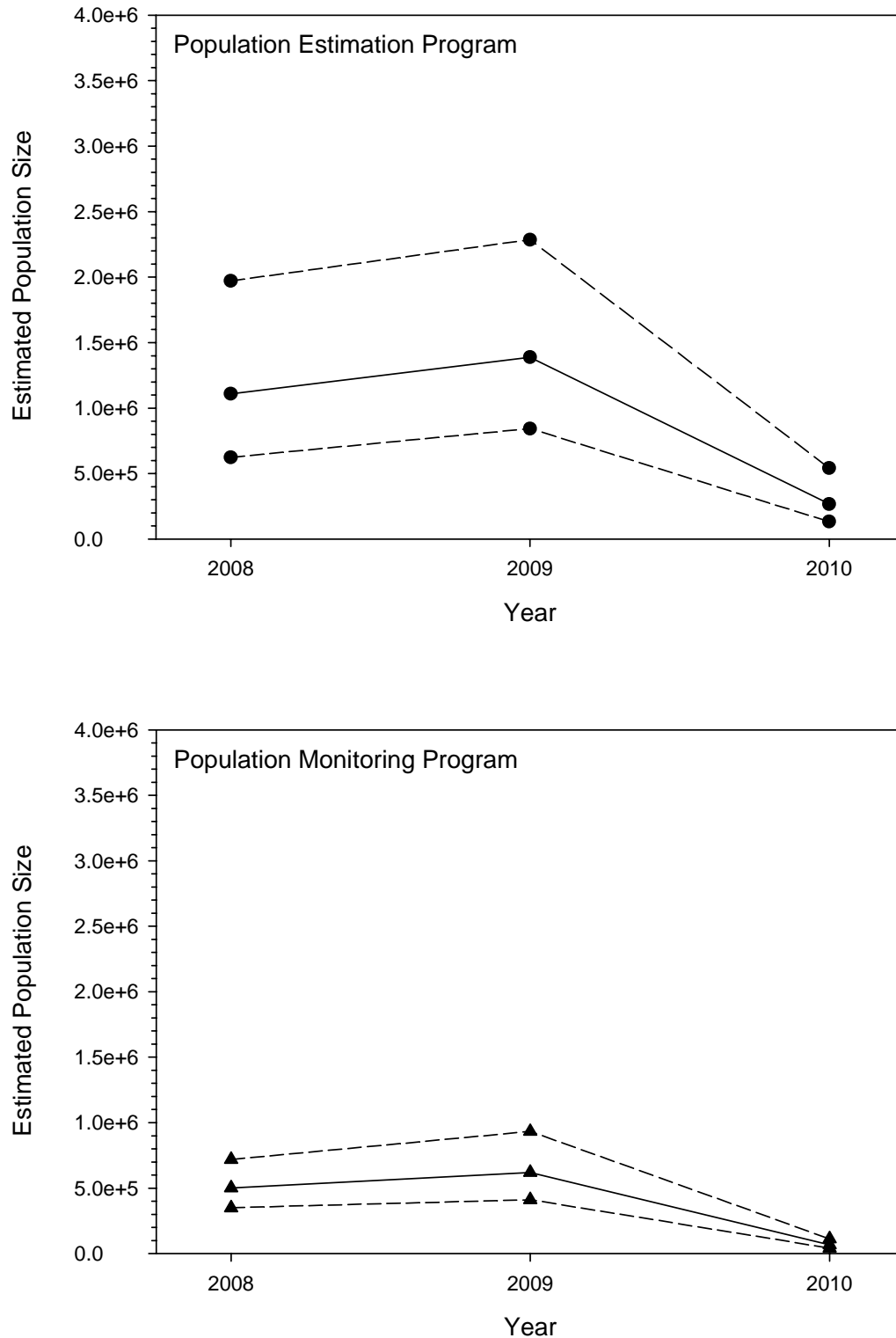
Figure 6. Estimates of Rio Grande silvery minnow population size (unmarked individuals only) calculated from Population Estimation Program and Population Monitoring Program data from 2008 to 2010 (solid line shows estimate and dashed lines show 95% upper and lower confidence bounds).
