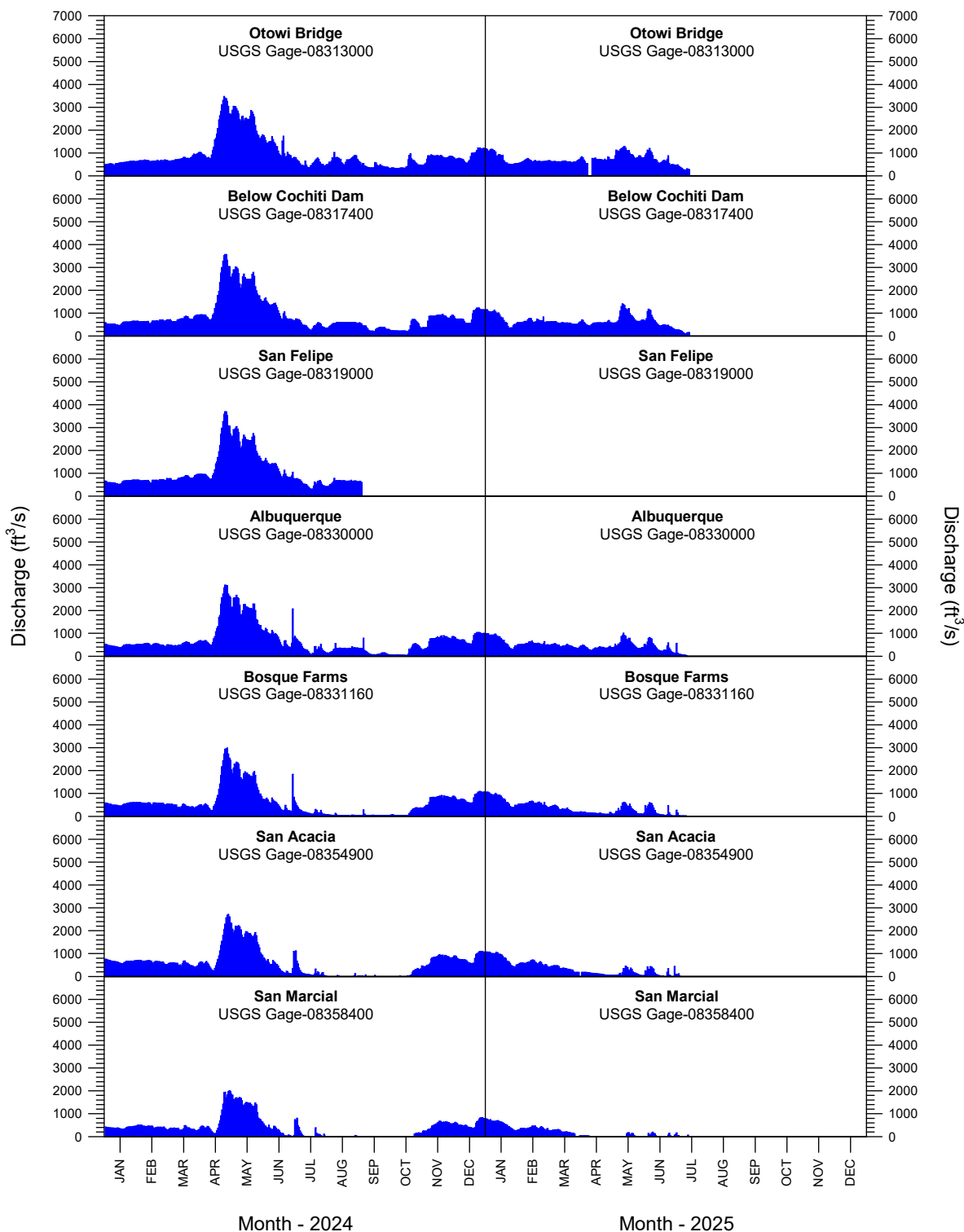
Figure 3. Rio Grande mean-daily discharge, by USGS gaging station, from 1 January 2024 to 15 July 2025. All discharge data are provisional and subject to change.
