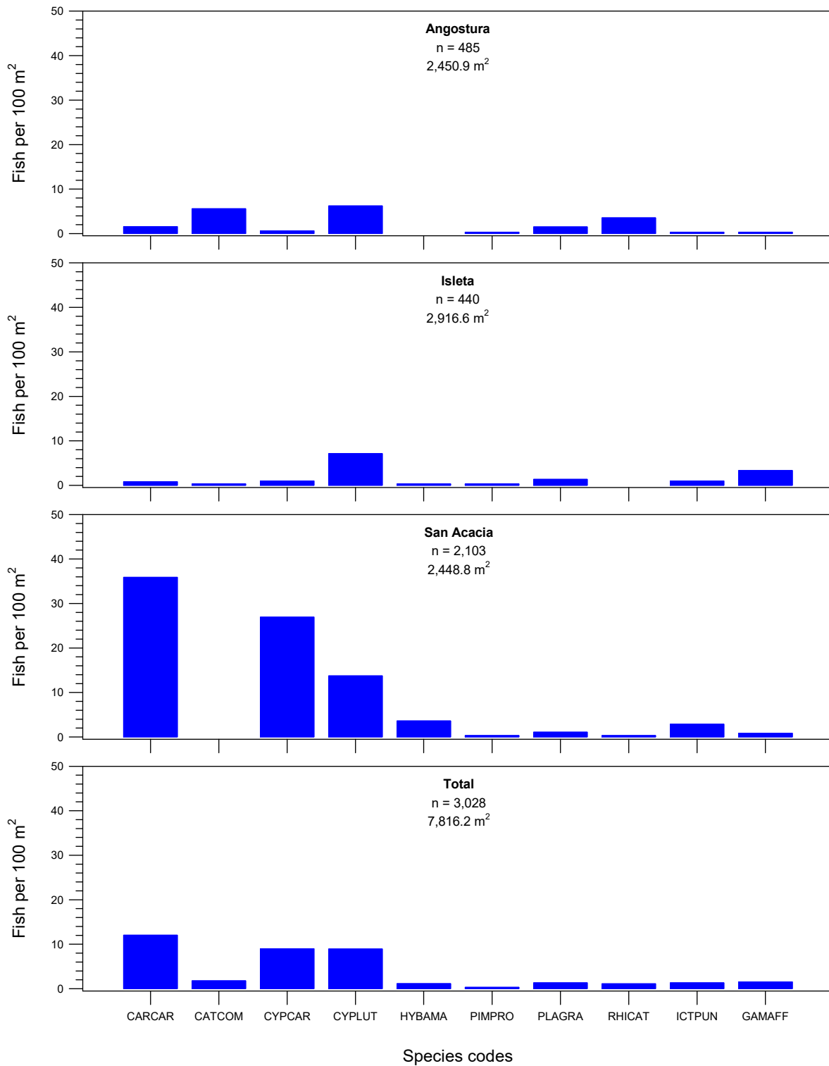
Figure 5. Fish densities based on all sites, by reach and focal taxa, during June 2025. Marked and unmarked Rio Grande Silvery Minnow were included.
